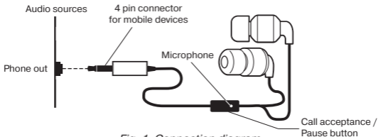
Fig. 1. Connection diagram
