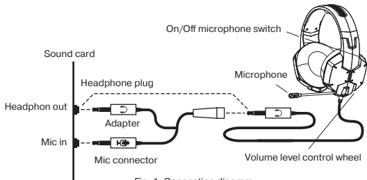
Fig. 1. Connection diagram
